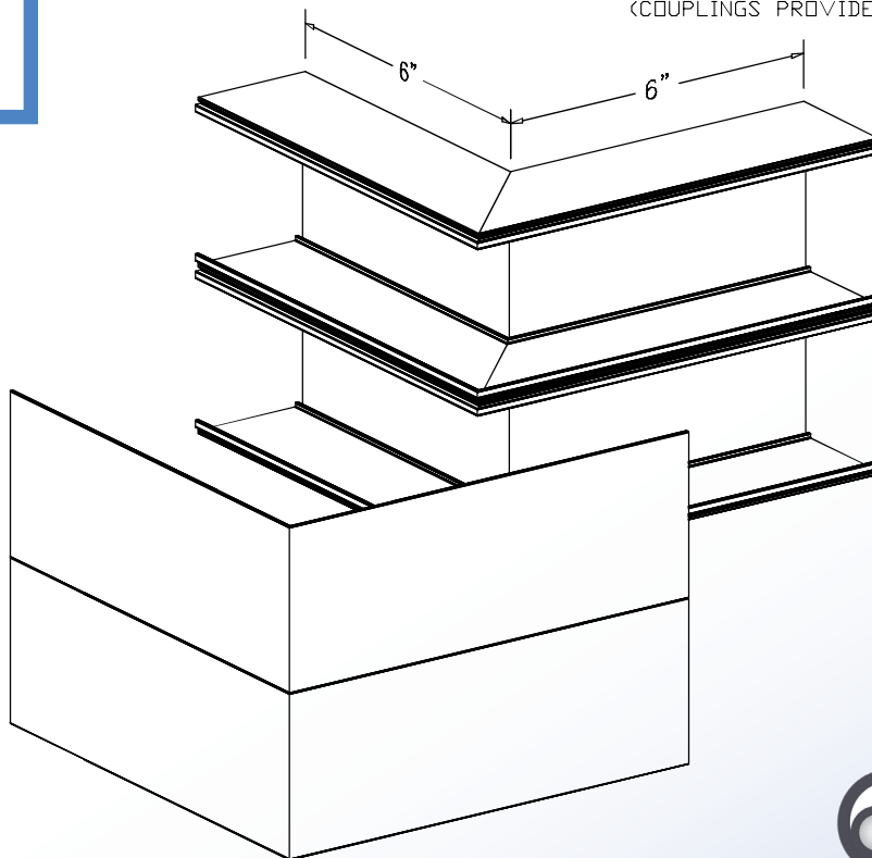
SWA4818 - FITTING AND COVER (COUPLINGS PROVIDED FOR RACEWAY ATTACHMENT)
