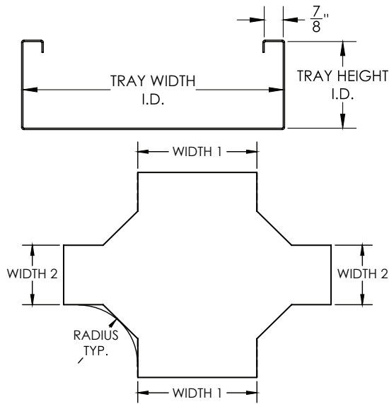
SBX-COVX-RHC-XXXX-XX REDUCING HORIZONTAL CROSS COVER
