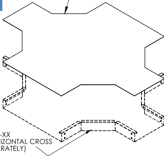
SBX-COVX-RHC-XXXX-XX REDUCING HORIZONTAL CROSS COVER
