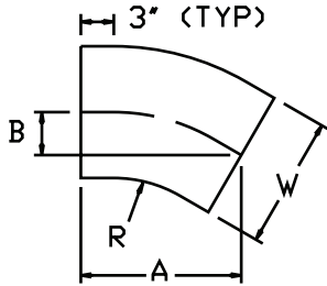
30° ELBOW
