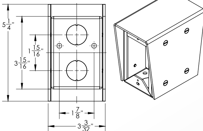
DPS-1-DM (2) 1-GANG, BACK TO BACK ALUMINUM DESK PEDESTAL
