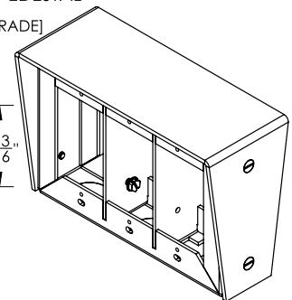
DPS1-3-DM 3-GANG, SINGLE SIDED ALUMINUM DESK PEDESTAL
