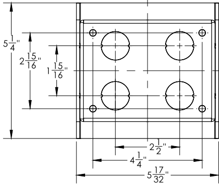
DPS-2-DM (2) 2-GANG, BACK TO BACK ALUMINUM DESK PEDESTAL
