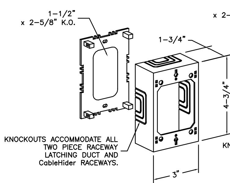
M.S.I. P/N: SWP2348 SINGLE GANG BOX
