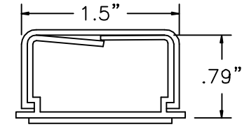
P/N: FWH-15060 BASE
