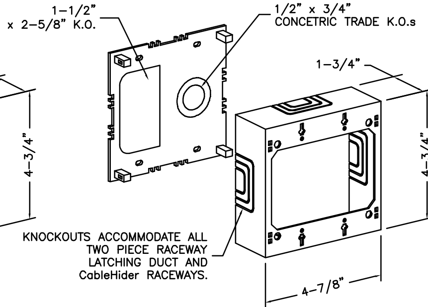
M.S.I. P/N: SWP2348-2 TWO GANG BOX
