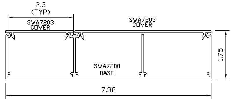
SWA7200 SERIES ALUMINUM RACEWAY SECTION VIEW SATIN ANNOIDIZED FINISH (EACH ORDERED SEPARATELY)
